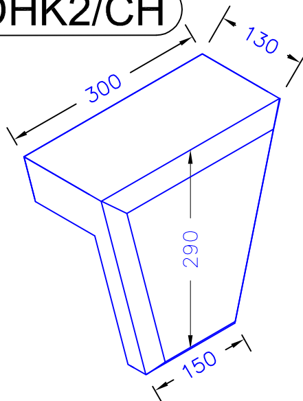
Clip Over Keystone Chamfered 300 x 130 x 290 9.90kg
