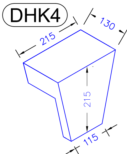
Clip Over Keystone 215 x 130 x 215
