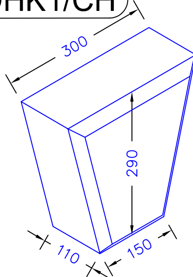
Chamfered Keystone 300 x 110 x 290 15.10kg
