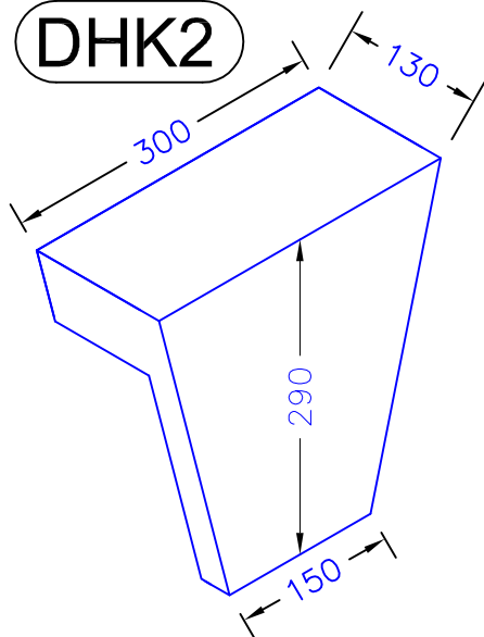
Clip Over Keystone 300 x 130 x 290 9.90kg
