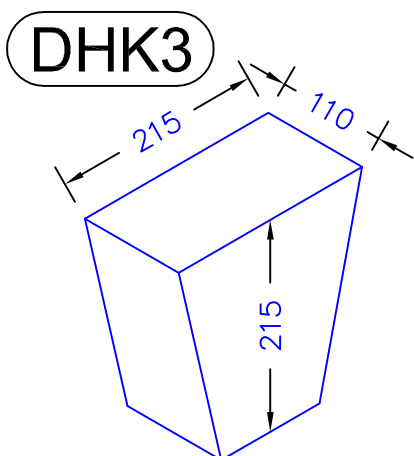
Plain Keystone 215 x 110 x 215
