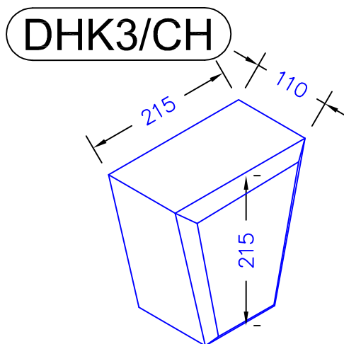
Chamfered Keystone 215 x 110 x 215
