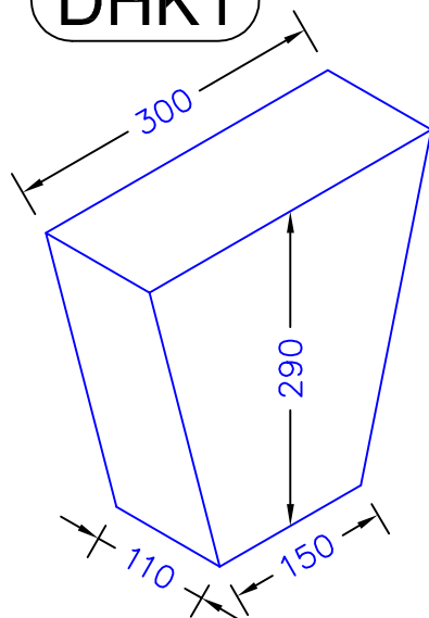
Plain Keystone 300 x 110 x 290 15.10kg
