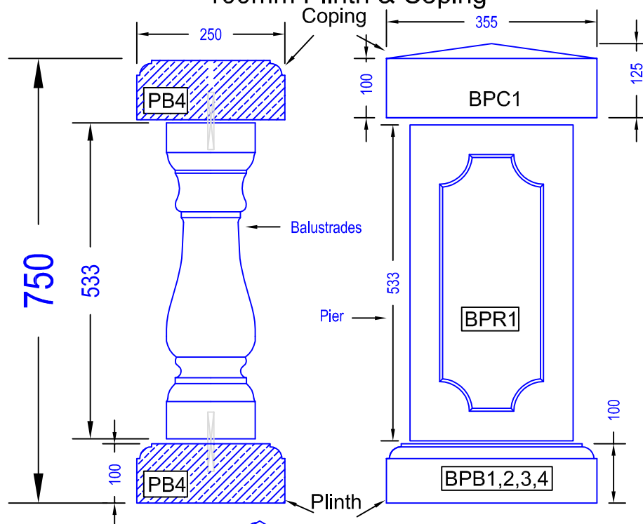
Balustrade 533mm high with 100mm Plinth & Coping
